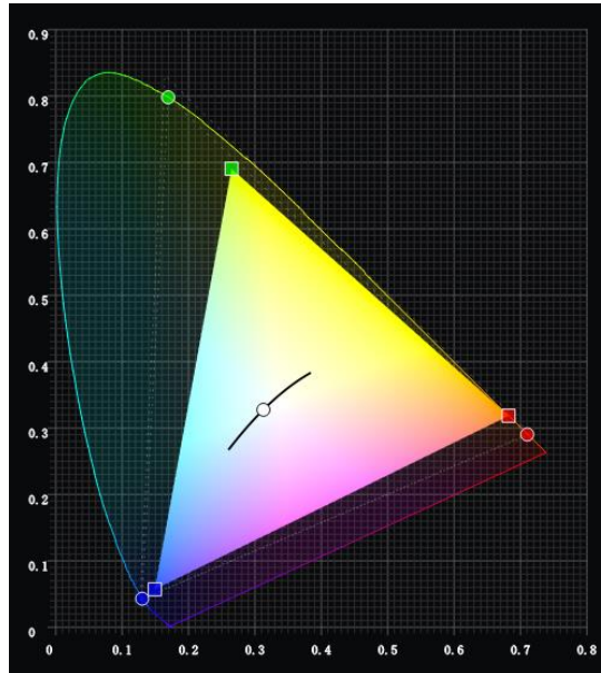
Figure 12.1-2 Horsehoe diagram
